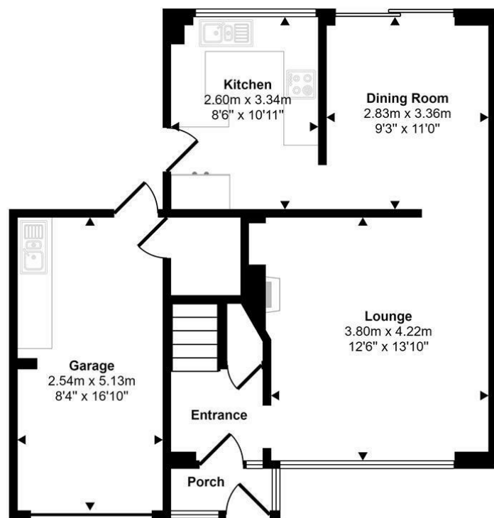
Ground Floor Approx 58 sq m / 629 sq ft
